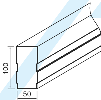
BEAM SECTION 100x50
