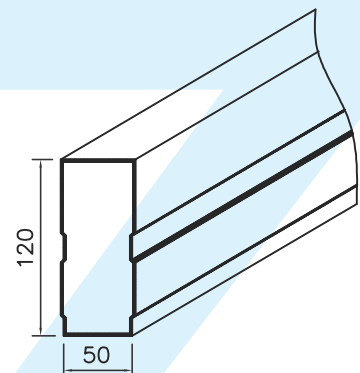
BEAM SECTION 120x50
